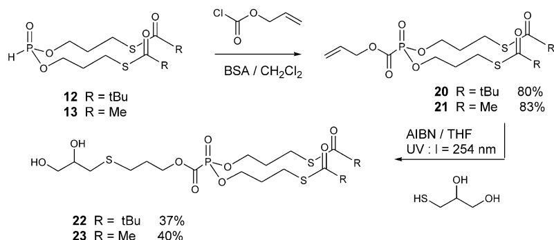
Figure 9. Synthesis of thioglycerol derivatives.
