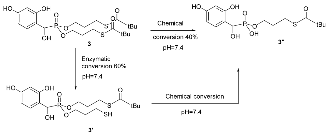
Figure 2. Decomposition process of model compound 3 .
