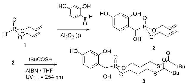
Figure 1. Reaction scheme for model compound.
