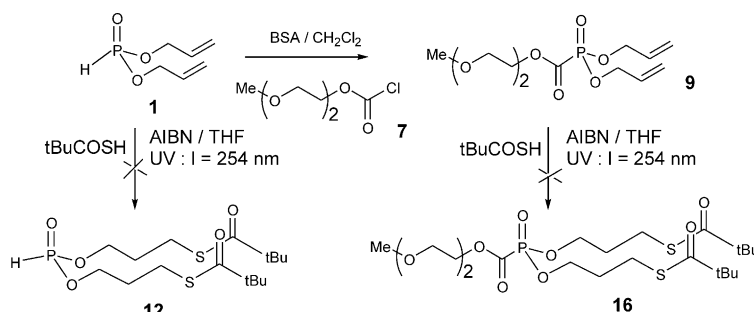
Figure 6. The direct syntheses of Bis SATP phosphonate fail.
