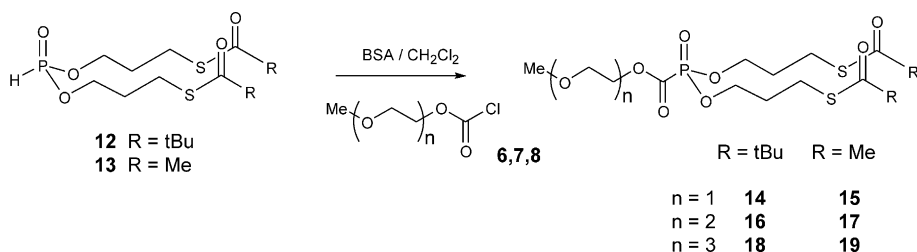
Figure 8. Reaction scheme for Bis (RSATP) polyethyleneglycol monomethylether phosphonoformates.
