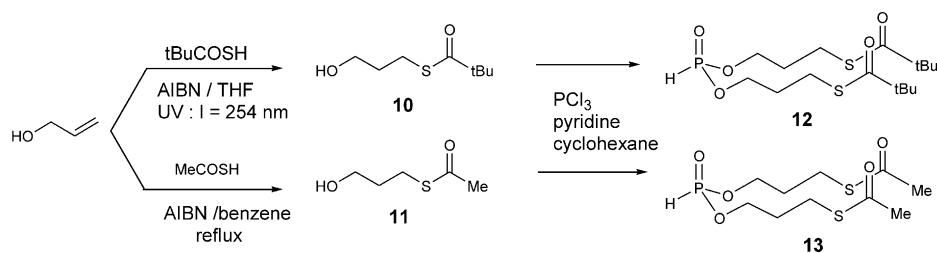
Figure 7. Reaction scheme for the bis enzyme-labile phosphonates.
