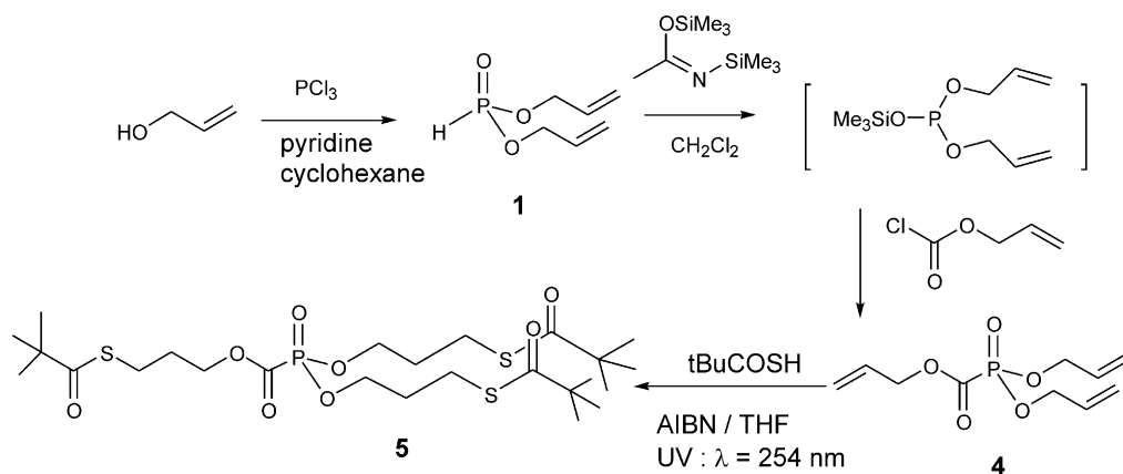
Figure 4. Synthesis of tris ( S -pivaloyl-3-thiopropyl)phosphonoformate 5 .
